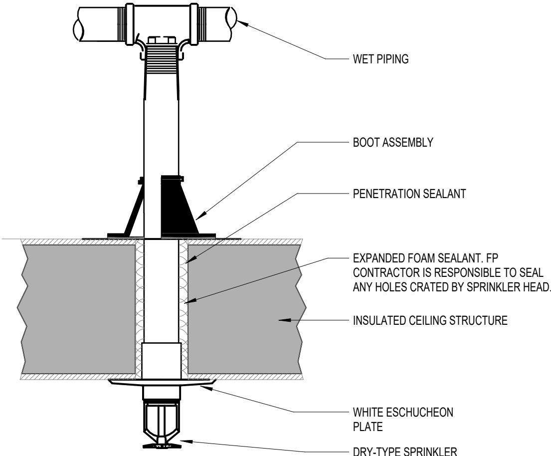
E5 DRY-TYPE SPRINKLER INSTALLATION NOT TO SCALE
