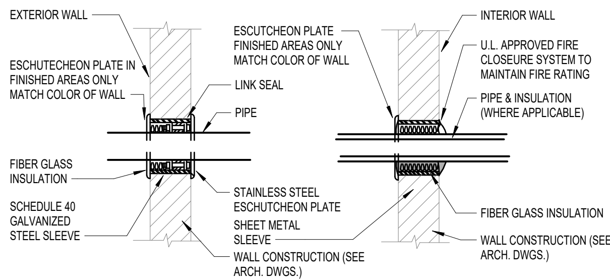
E3 WALL PENETRATION NOT TO SCALE
